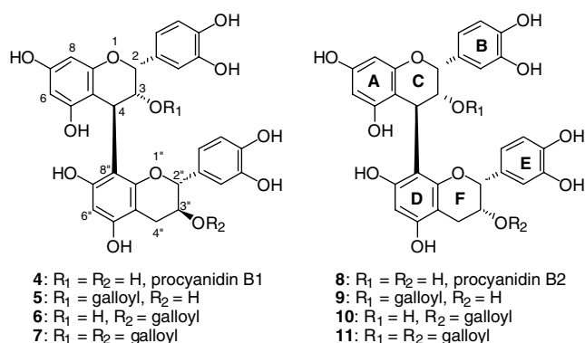
Figure 2. Structures of galloyl-substituted procyanidin B1 and procyanidin B2.
