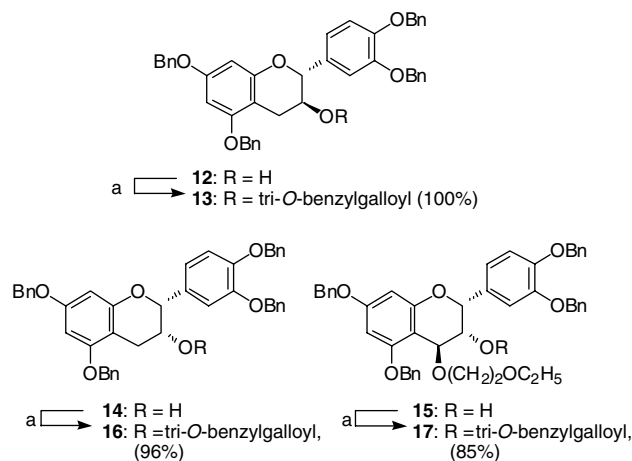
Scheme 1. Synthesis of tri- O -benzylgalloyl catechin ( 13 ) and tri- O -benzylgalloyl epicatechin derivatives ( 16 ) and ( 17 ). Reagents: (a) DCC, DMAP, CH 2 Cl 2 .
