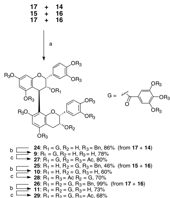
Scheme 3. Synthesis of 3- O -galloyl-substituted procyanidin B2 series. Reagents: (a) TMSOTf, CH 2 Cl 2 ; (b) Pd(OH) 2 /C, H 2 , THF/MeOH/H 2 O; (c) Ac 2 O, py, DMAP.
