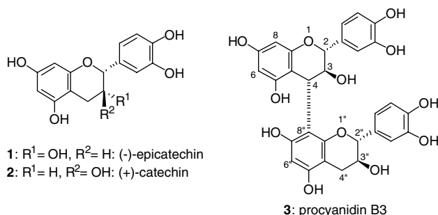
Figure 1. Structures of (-)-epicatechin (1), (+)-catechin (2), and procyanidin B3 (3).
