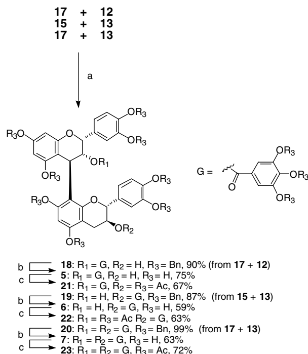
Scheme 2. Synthesis of 3- O -galloyl-substituted procyanidin B1 series. Reagents: (a) TMSOTf, CH 2 Cl 2 ; (b) Pd(OH) 2 /C, H 2 , THF/MeOH/H 2 O; (c) Ac 2 O, py, DMAP.
